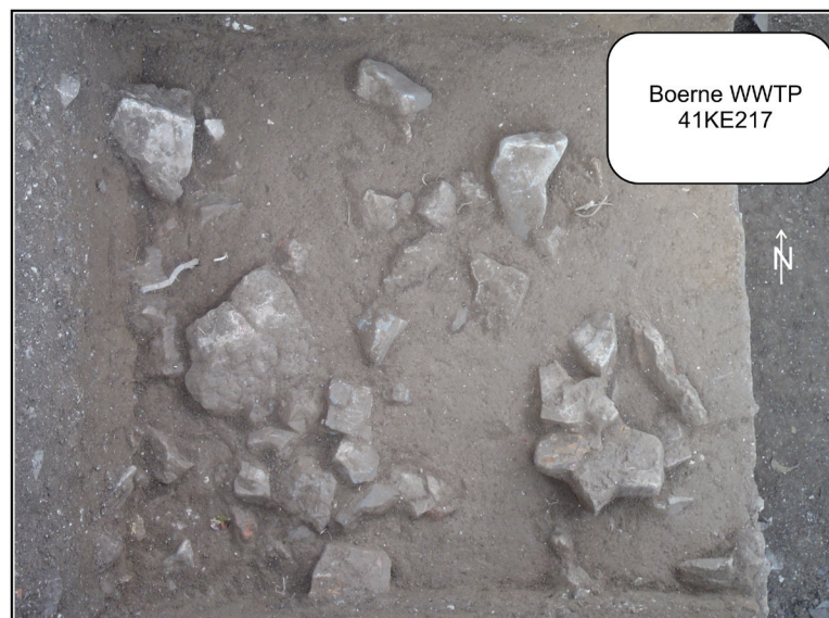
Figure 6-7. View of burned rock in lower depositional zone, TU 3 at 60 cmbs (23.6 in.).
