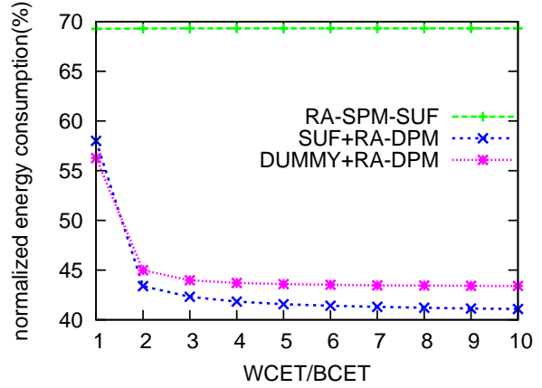
b. energy for U = 0.5 and p \in [10, 20]
