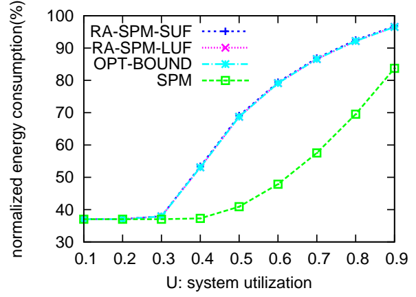
(b) 20 tasks with p \in [10, 20]
