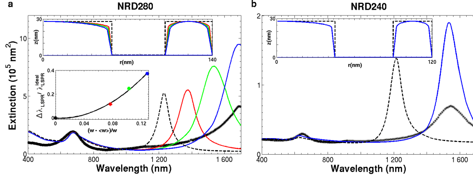
Fig. 4. Extinction spectra of NRD280 (a) and NRD240 (b) calculated for the various profiles of the ring-disks shown in the insets (only half the ring-disk is sketched). The spectrum corresponding to each profile is color-encoded. The profiles of the perfect ring-disks with sharp edges and flat surfaces and the corresponding spectra are shown in black dashed lines. The measured optical density spectra [ OD = -\log(T) ] are plotted with black dots. The inset in panel (a) shows the relative LSPR shift \Delta\lambda/\lambda_{LSPR}^{ideal} as a function of the relative deviation of the mean NR wall thickness (w - \langle w \rangle)/w .
